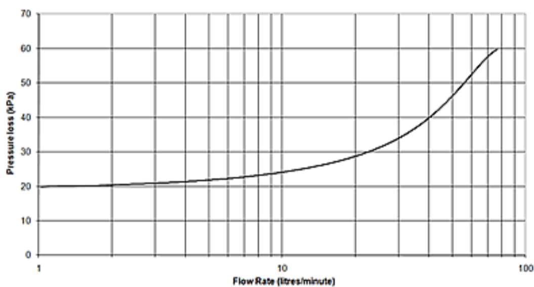
Pressure Loss Dual Check 16mm
